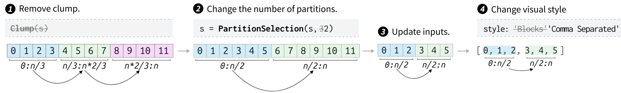
Figure 2: Variations on array partitions in Figure 1: 1 removes a simplification; 2 updates the number of partitions to two; 3 halves the length of the input list; and 4 updates the initial visual style to be a comma separated list instead of blocks.
