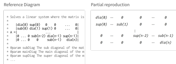
Figure 5: A Example gallery of reproduced diagrams. At the bottom are two diagrams whose abstraction Chisel was unable to capture, along with the partial reproduction: B A binary tree diagram, from MIT’s Introduction to Algorithms [13] shows a branch as part of a larger subtree, and C Tridiagonal matrix, from Chromium [9] which uses partial abbreviations on the rows.
